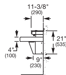
Side View (Both Two & Three Stations)
