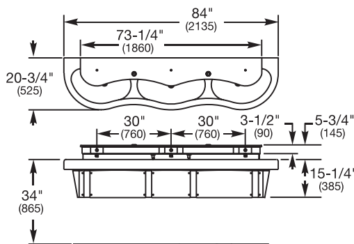
Three Station - Model 3793 (Top & Front View)
