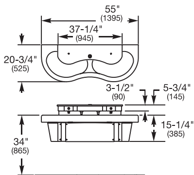
Two Station - Model 3792 (Top & Front View)
